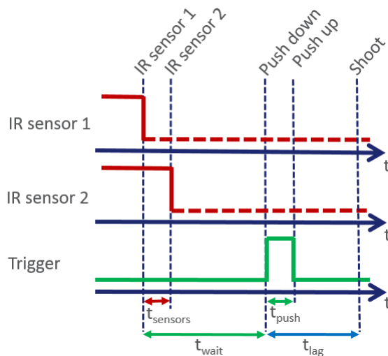
Figure 7. Timing diagram.
