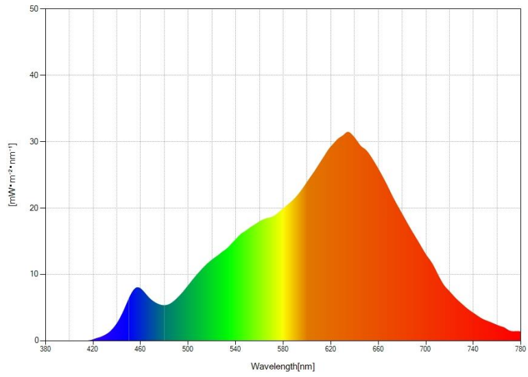
All LEDs ON spectrum (2600-2700K)
