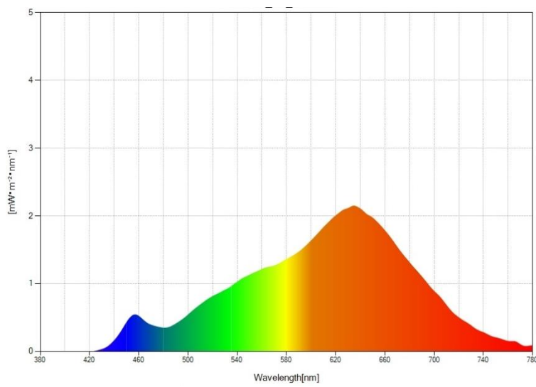
Low Light spectrum (2600-2700K)
