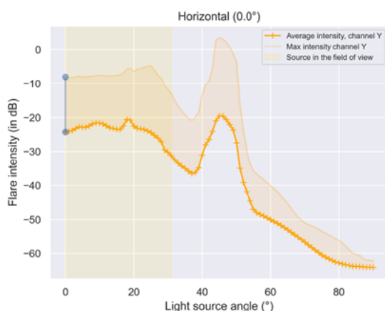
Example of evolution of flare as a function of light source angle
